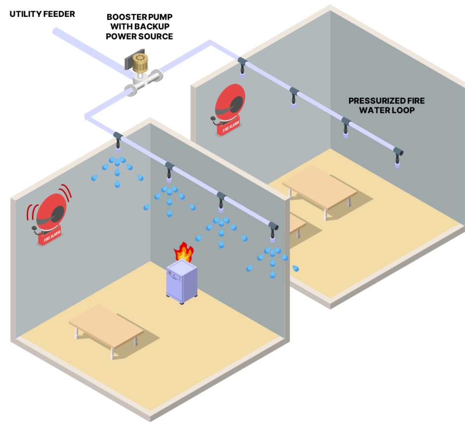
Figure 33: Example Fire Alarm and Fire Water System
